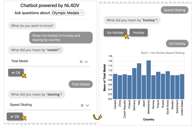
Figure 4: A chatbot where the system collaborates with the user to resolve ambiguities during query interpretation.
