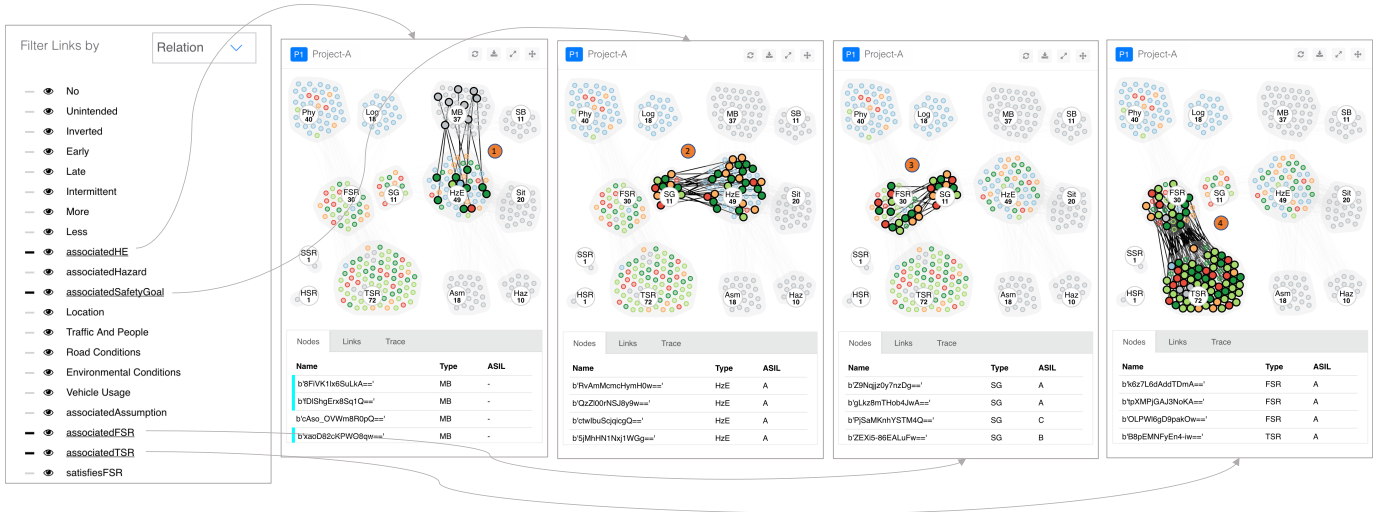
Fig. 8. Find Missing Links. (1) Each Malfunctioning Behavior (MB) should have a Hazardous Event (HZE). (2) Each HZE should have a Safety Goal (SG). (3) Each SG should define a Functional Safety Requirement (FSR). (4) Each FSR should define a Technical Safety Requirement (TSR).
