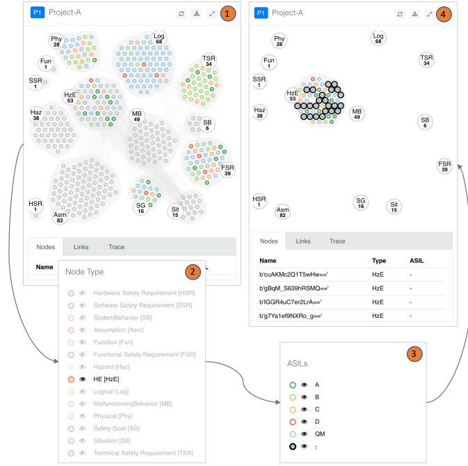
Fig. 7. Find elements that are not yet assigned an ASIL. (1) Default State where nodes are colored by their ASIL, (2) Deselect all Node Types except Hazardous Events (HzE), (3) Select all nodes with unassigned ASILs, and (4) The selected ASILs are highlighted with a black border.
